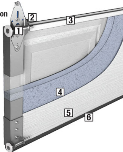
Steel Heritage Hinge
